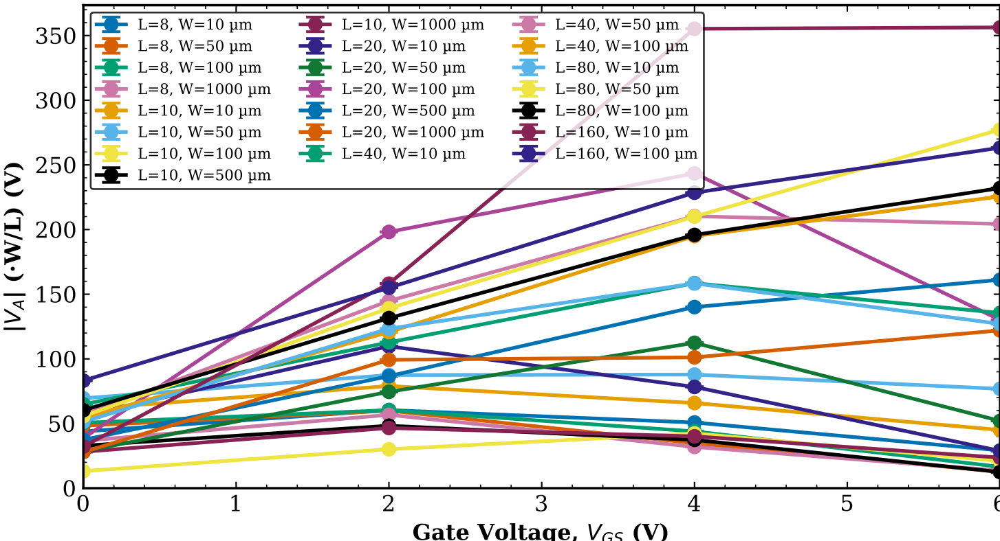
TFT1 Transistor 2 Early Voltage |V_A| vs V_G
